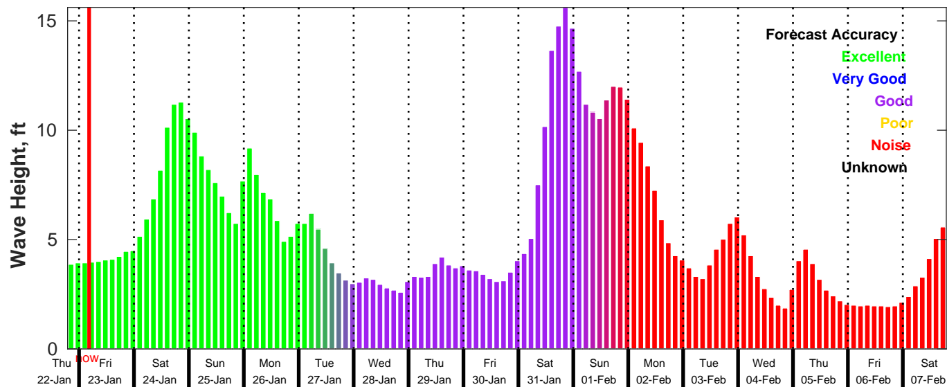
GFS Wave Forecast for NDBC 41004 from 22-Jan-2026 19:00:00 to 07-Feb-2026 19:00:00
