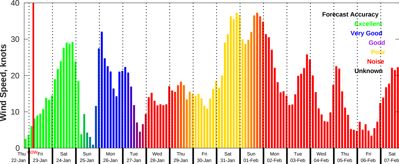
GFS Wind Speed Forecast for NDBC 41004 from 22-Jan-2026 19:00:00 to 07-Feb-2026 19:00:00
