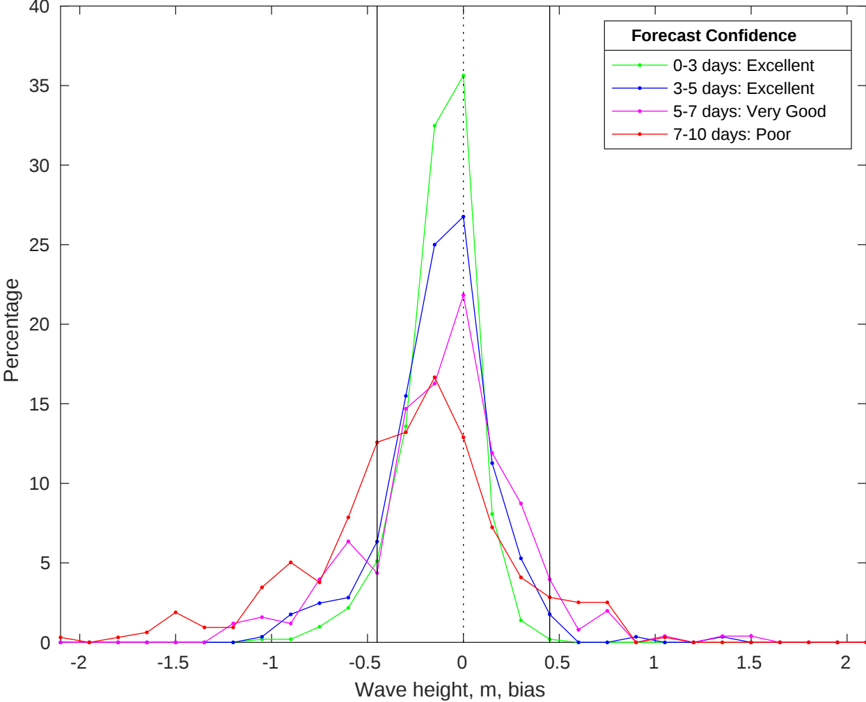
NDBC 41013 vs CMEMS Waves Bias Histogram: 23-Jan-2026
