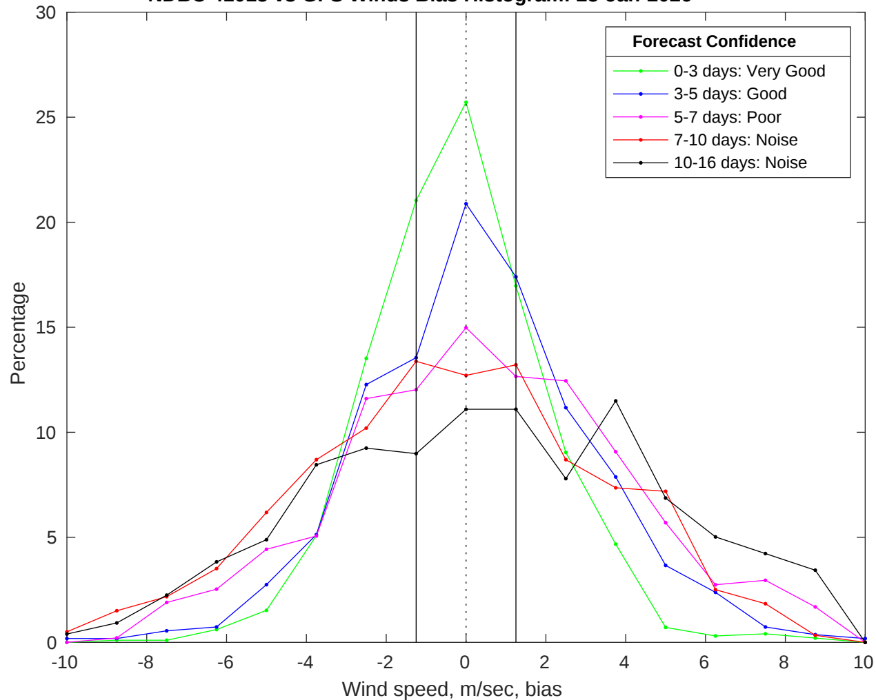
NDBC 41013 vs GFS Winds Bias Histogram: 23-Jan-2026
