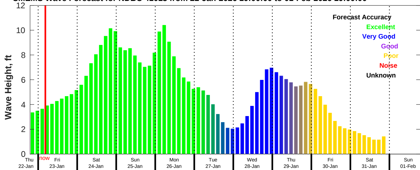
CMEMS Wave Forecast for NDBC 41013 from 22-Jan-2026 19:00:00 to 01-Feb-2026 19:00:00
