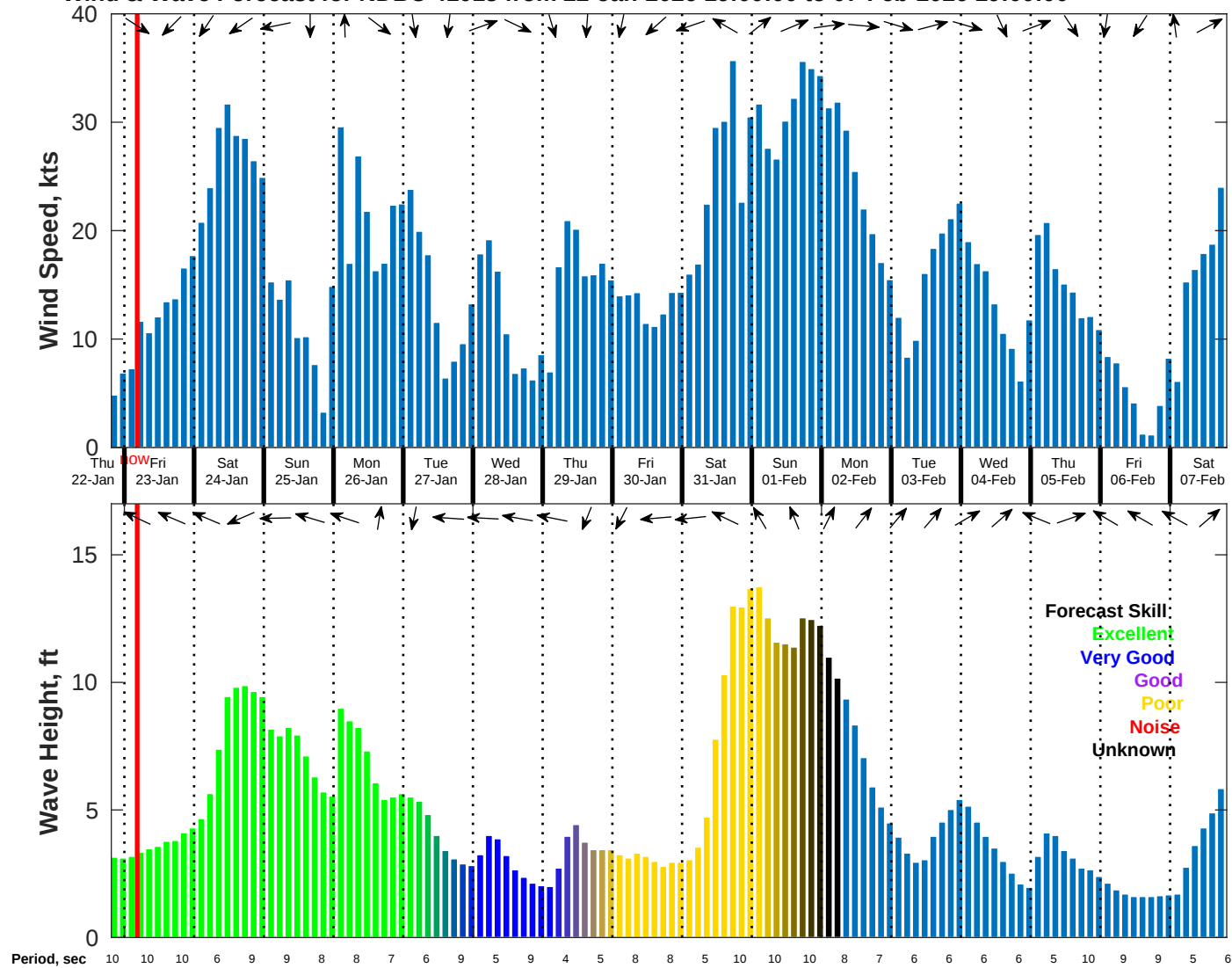
Wind & Wave Forecast for NDBC 41013 from 22-Jan-2026 19:00:00 to 07-Feb-2026 19:00:00
