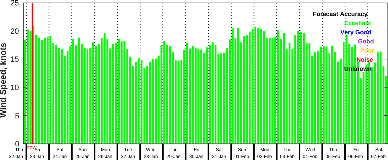
GFS Wind Speed Forecast for NDBC 41040 from 22-Jan-2026 21:00:00 to 07-Feb-2026 21:00:00
