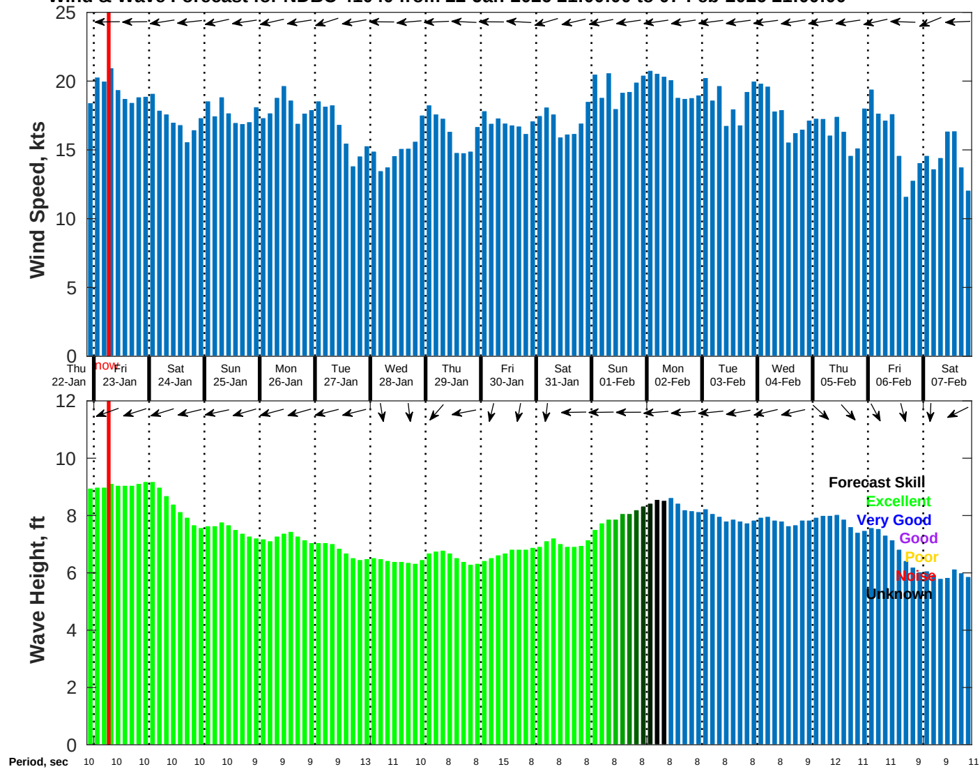
Wind & Wave Forecast for NDBC 41040 from 22-Jan-2026 21:00:00 to 07-Feb-2026 21:00:00
