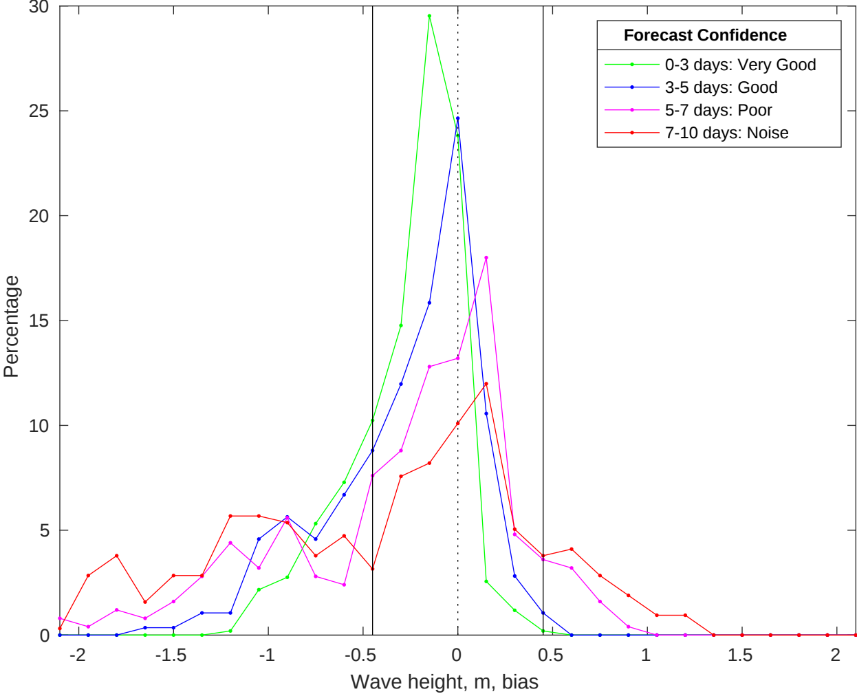
NDBC 42019 vs CMEMS Waves Bias Histogram: 23-Jan-2026
