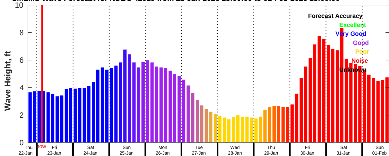
CMEMS Wave Forecast for NDBC 42019 from 22-Jan-2026 18:00:00 to 01-Feb-2026 18:00:00
