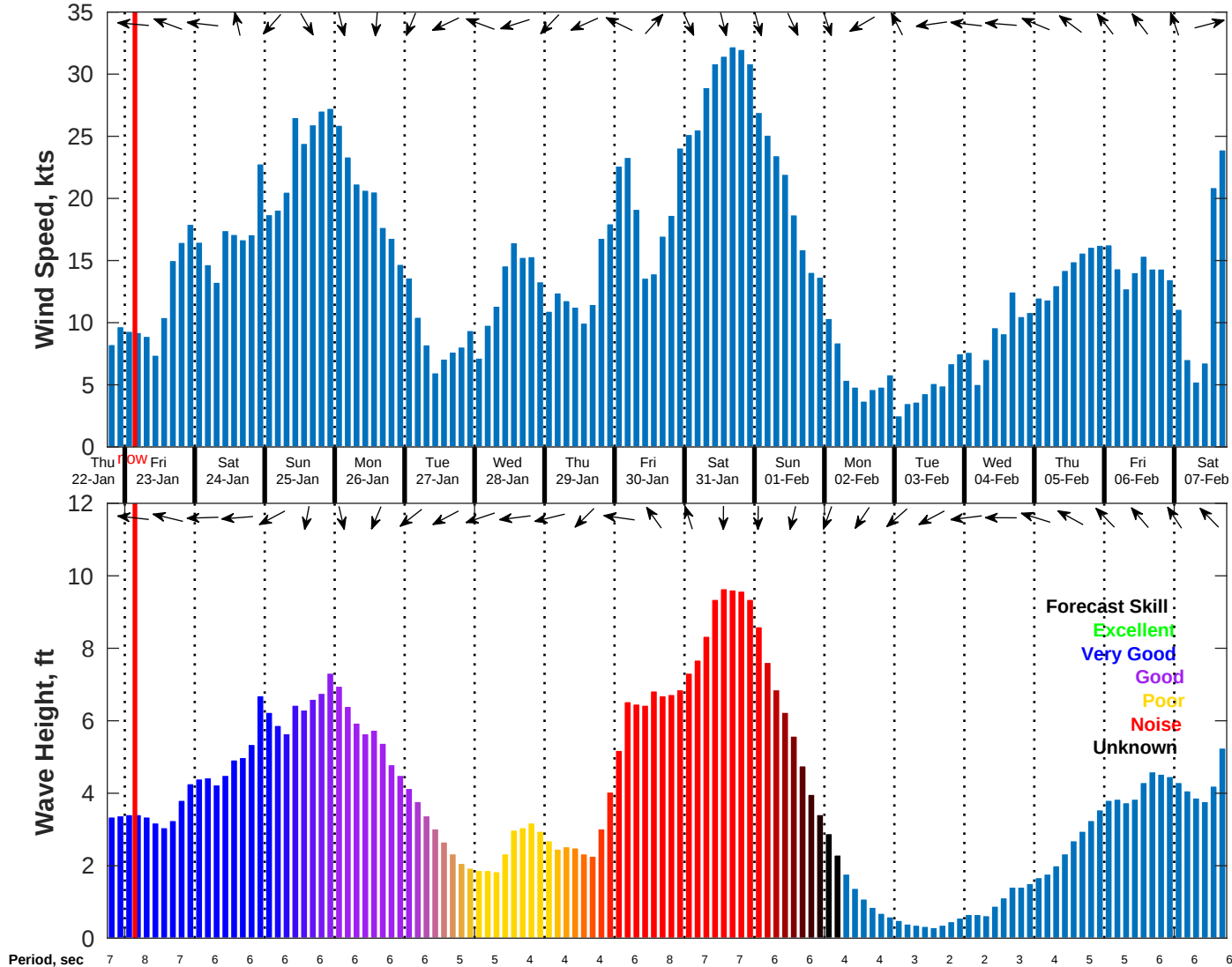
Wind & Wave Forecast for NDBC 42019 from 22-Jan-2026 18:00:00 to 07-Feb-2026 18:00:00
