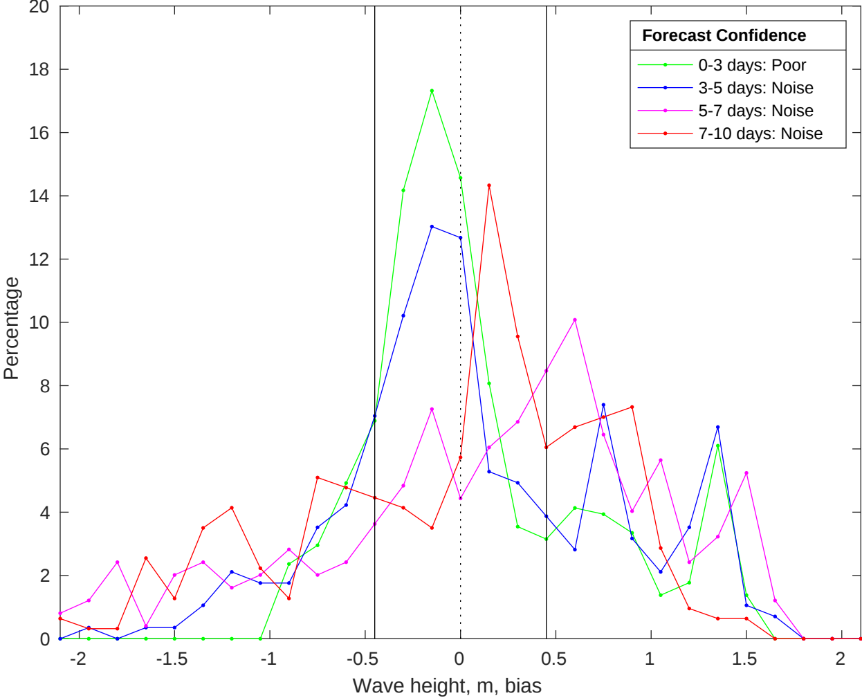
NDBC 42020 vs CMEMS Waves Bias Histogram: 23-Jan-2026
