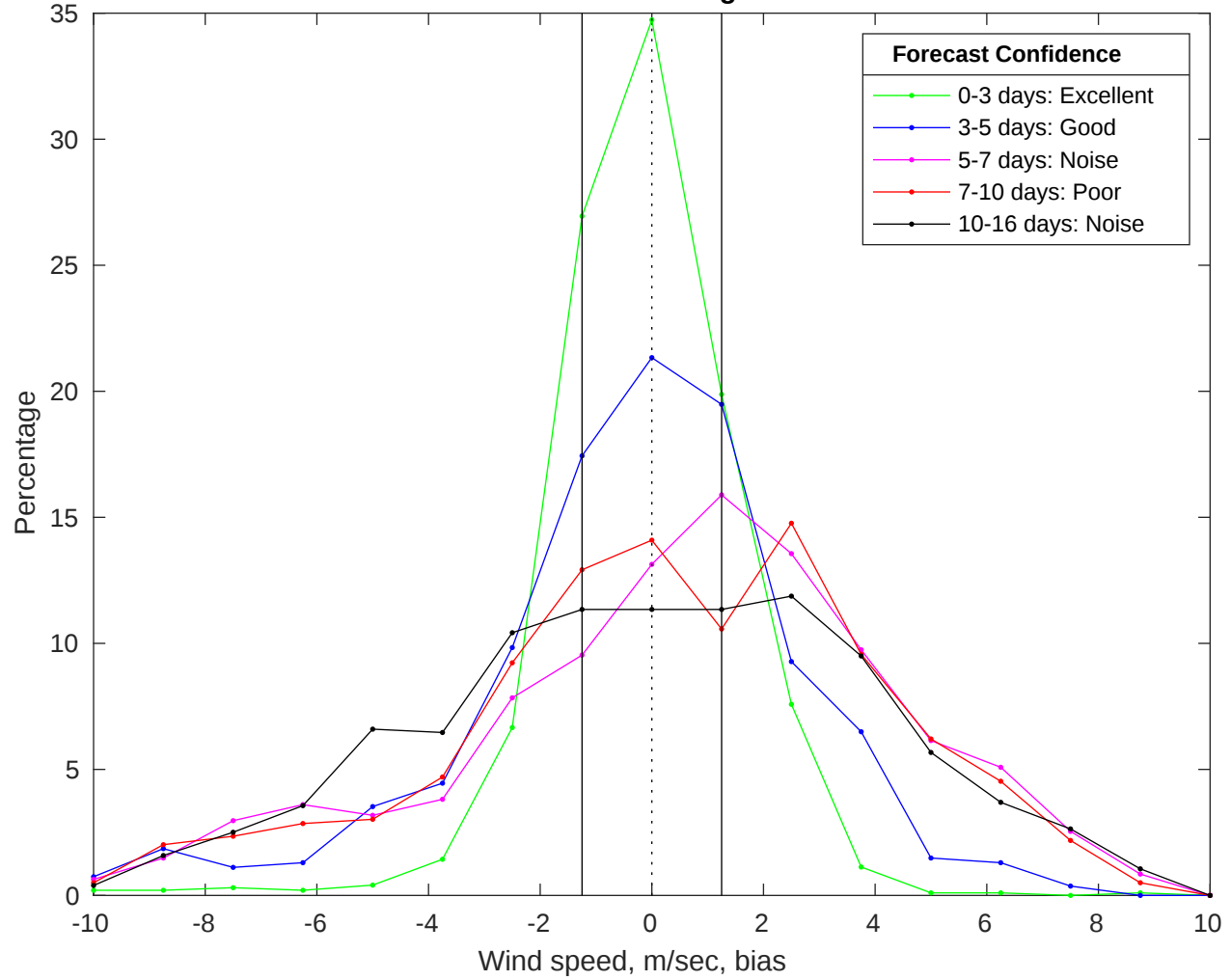
NDBC 42020 vs GFS Winds Bias Histogram: 23-Jan-2026
