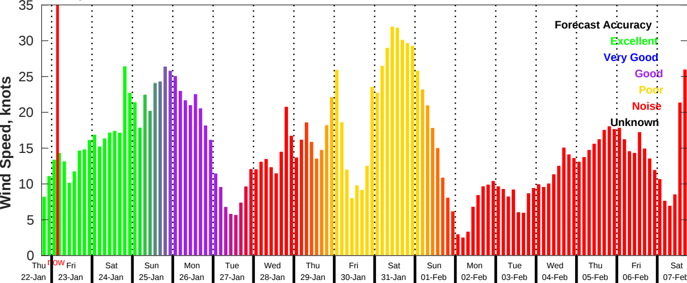
GFS Wind Speed Forecast for NDBC 42020 from 22-Jan-2026 18:00:00 to 07-Feb-2026 18:00:00
