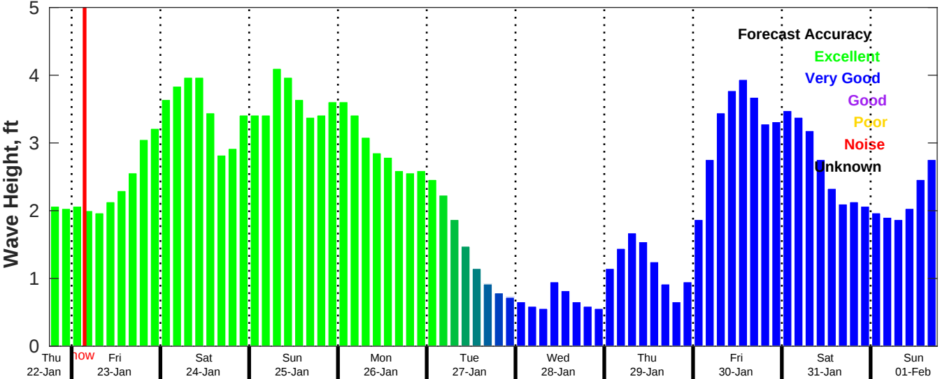
CMEMS Wave Forecast for NDBC 42035 from 22-Jan-2026 18:00:00 to 01-Feb-2026 18:00:00
