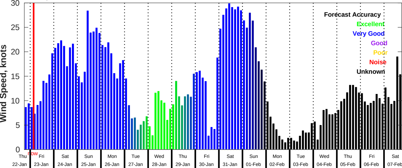
GFS Wind Speed Forecast for NDBC 42035 from 22-Jan-2026 18:00:00 to 07-Feb-2026 18:00:00
