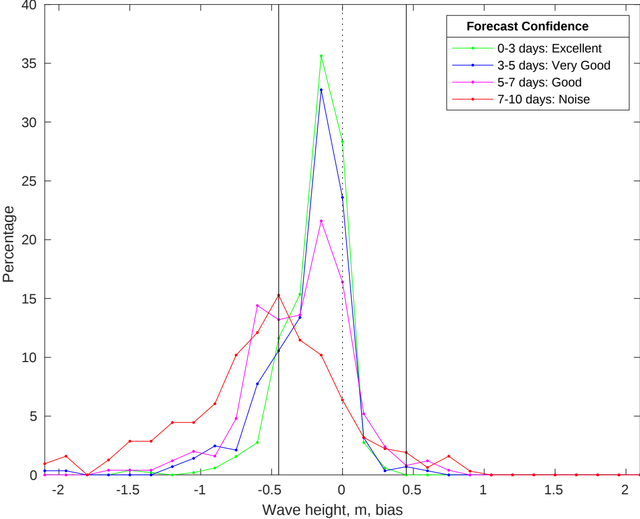
NDBC 42036 vs CMEMS Waves Bias Histogram: 23-Jan-2026
