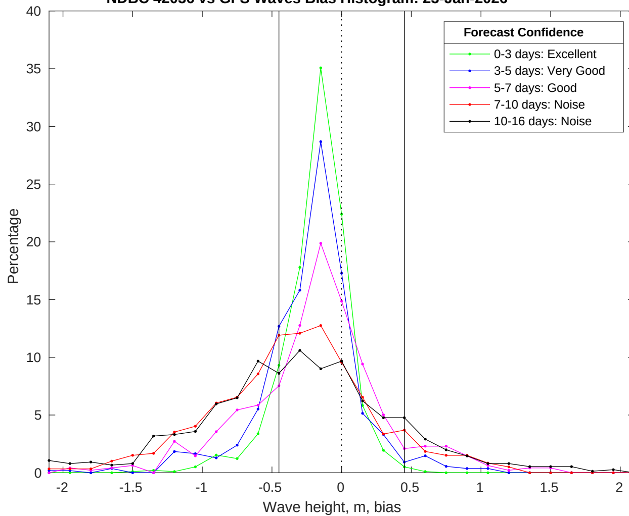
NDBC 42036 vs GFS Waves Bias Histogram: 23-Jan-2026
