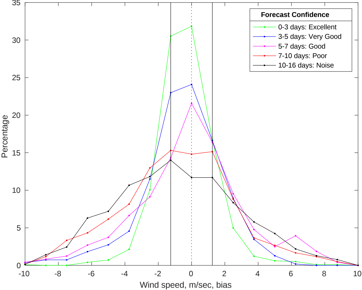
NDBC 42036 vs GFS Winds Bias Histogram: 23-Jan-2026
