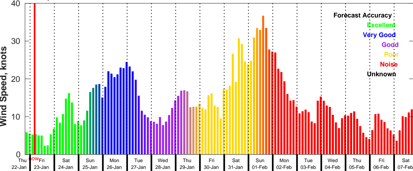
GFS Wind Speed Forecast for NDBC 42036 from 22-Jan-2026 19:00:00 to 07-Feb-2026 19:00:00
