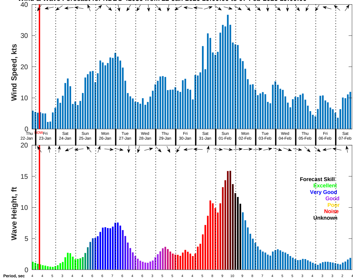
Wind & Wave Forecast for NDBC 42036 from 22-Jan-2026 19:00:00 to 07-Feb-2026 19:00:00
