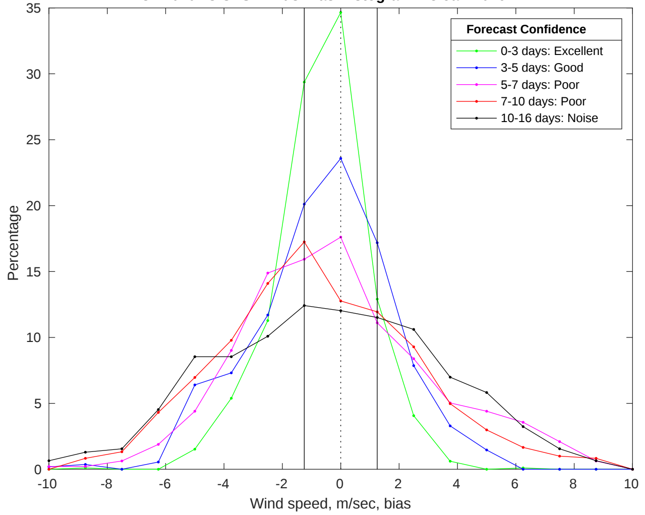
NDBC 42040 vs GFS Winds Bias Histogram: 23-Jan-2026
