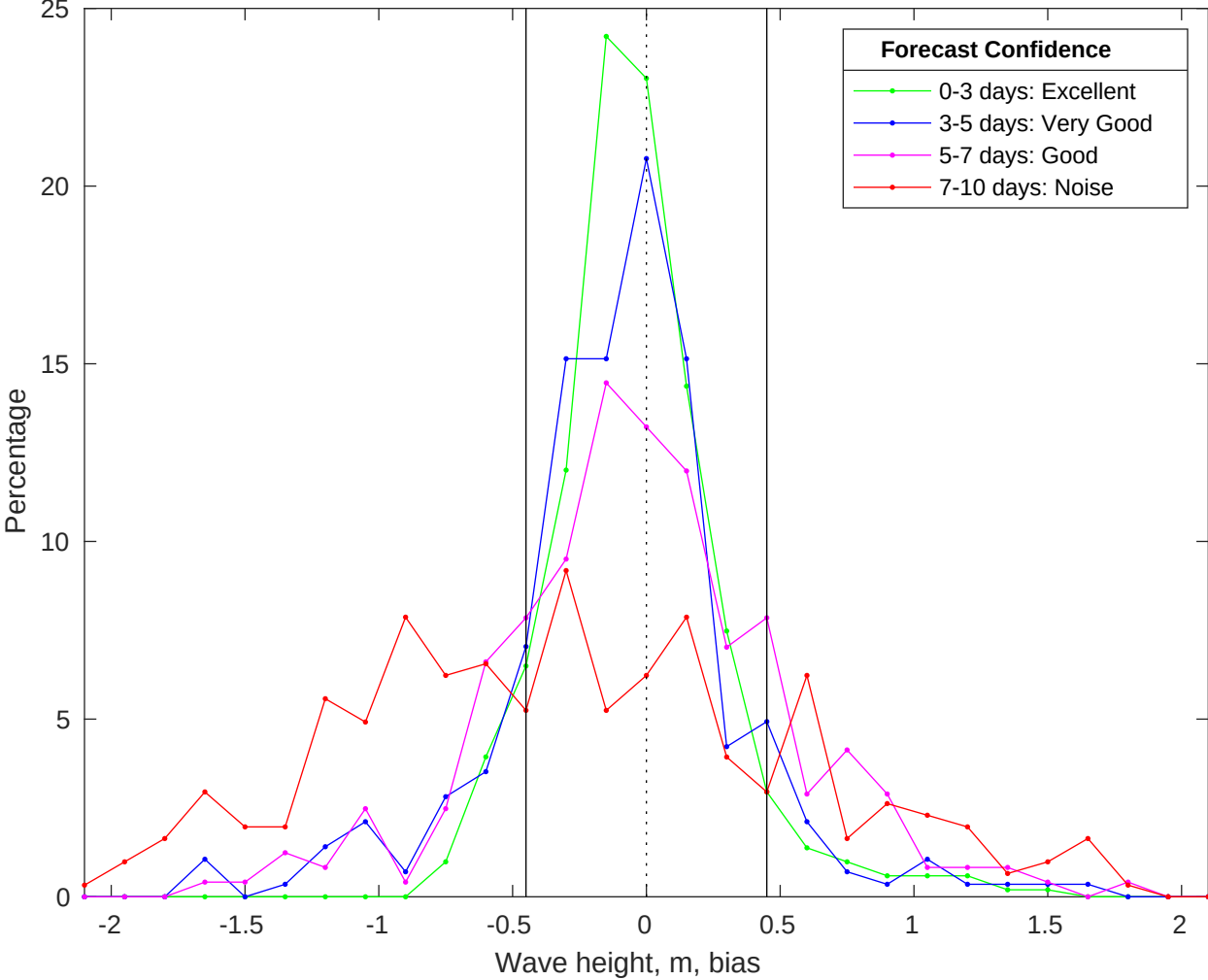
NDBC 44008 vs CMEMS Waves Bias Histogram: 23-Jan-2026
