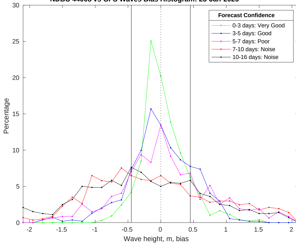
NDBC 44008 vs GFS Waves Bias Histogram: 23-Jan-2026
