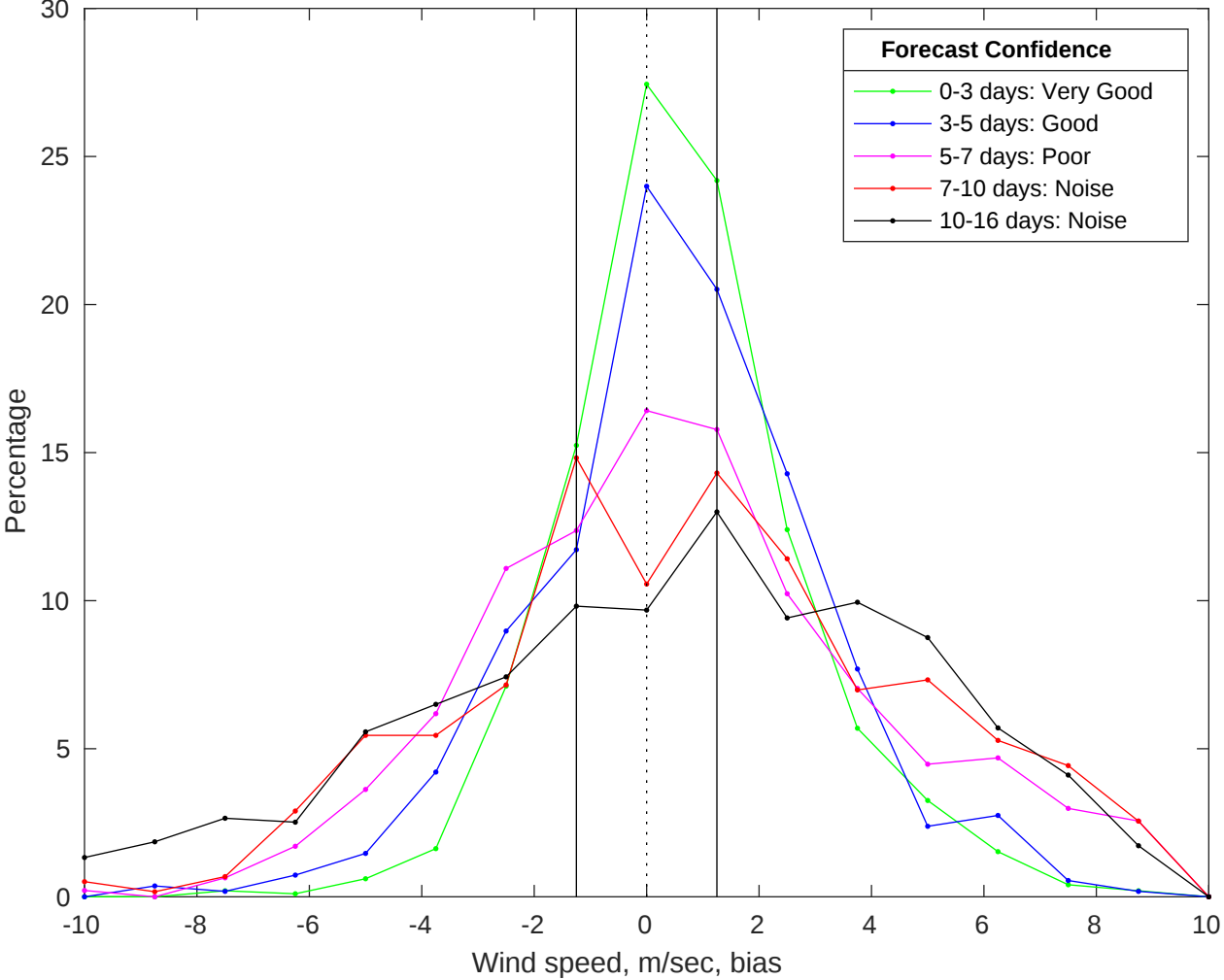
NDBC 44008 vs GFS Winds Bias Histogram: 23-Jan-2026
