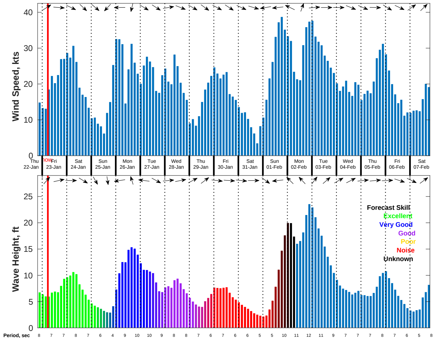
Wind & Wave Forecast for NDBC 44008 from 22-Jan-2026 20:00:00 to 07-Feb-2026 20:00:00
