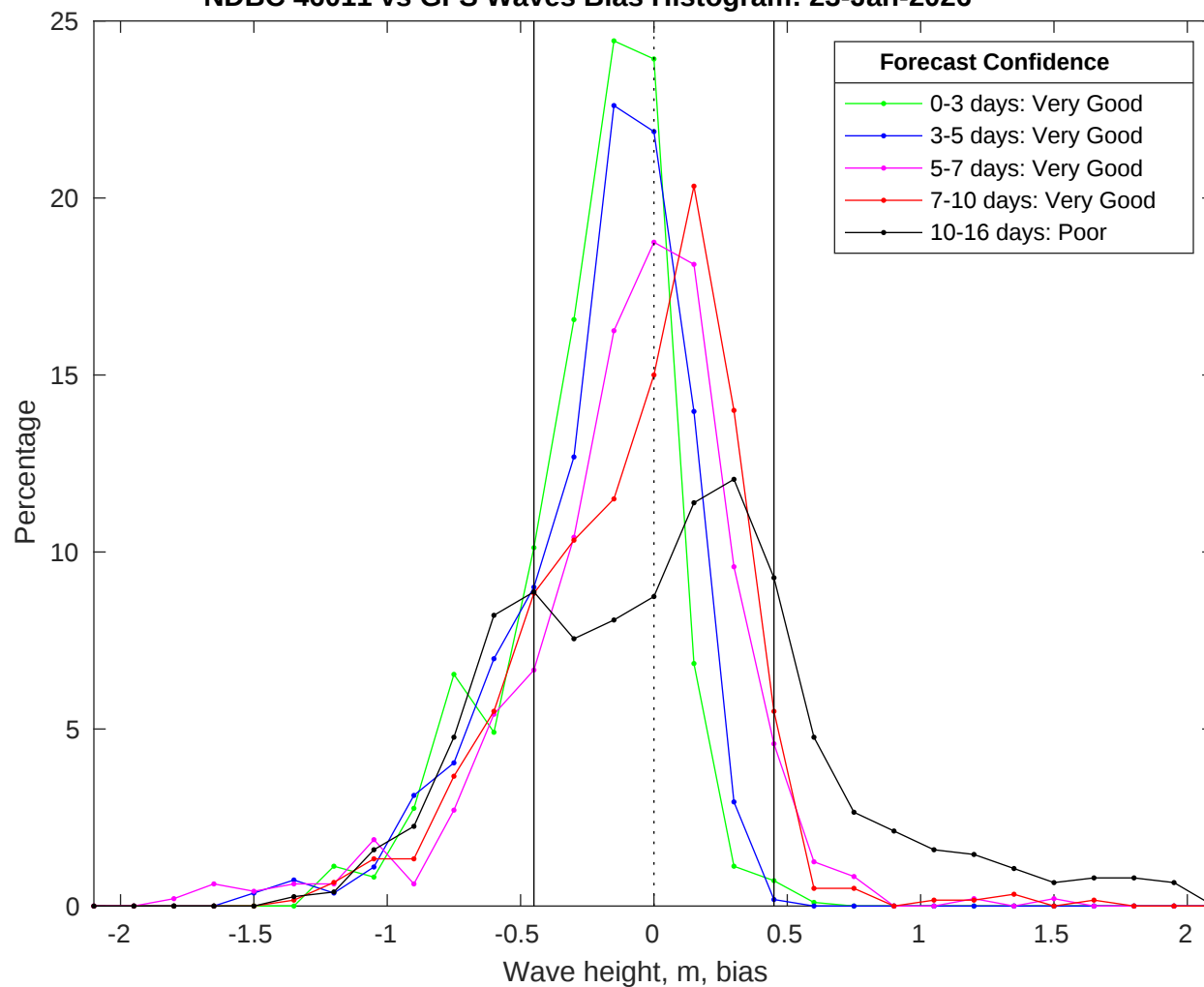
NDBC 46011 vs GFS Waves Bias Histogram: 23-Jan-2026
