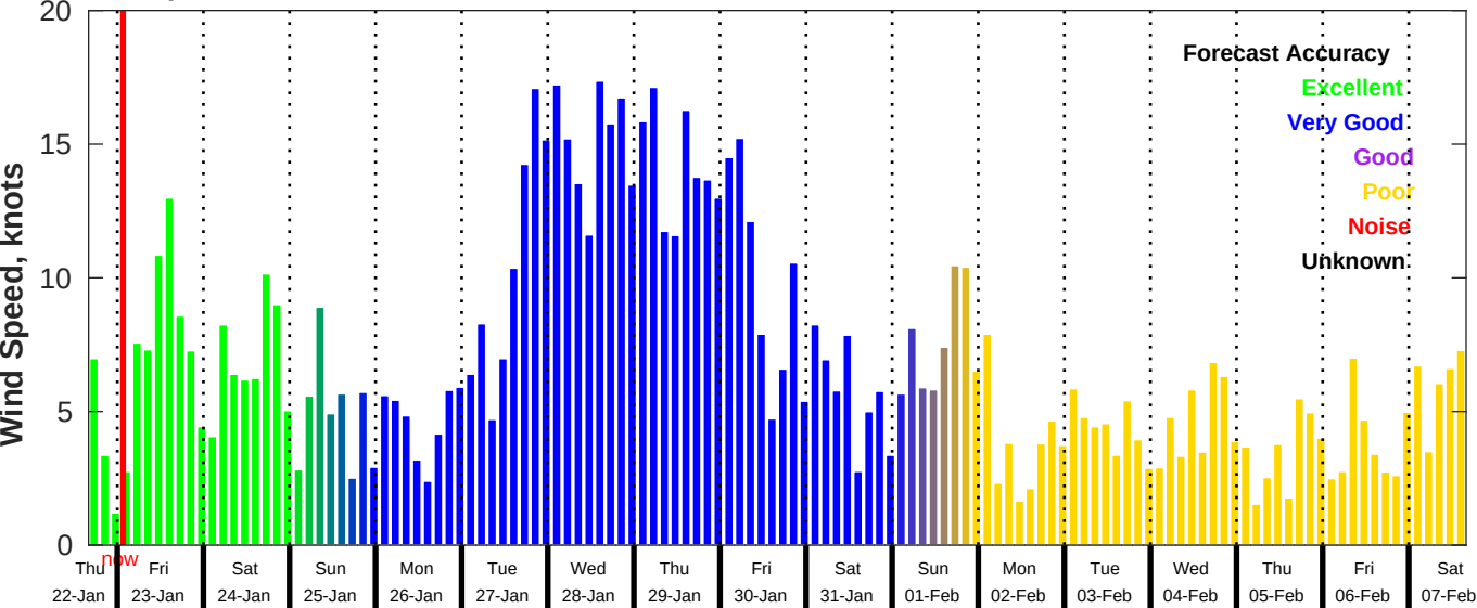
GFS Wind Speed Forecast for NDBC 46011 from 22-Jan-2026 16:00:00 to 07-Feb-2026 16:00:00
