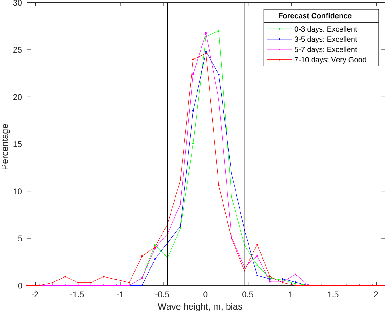
NDBC 46028 vs CMEMS Waves Bias Histogram: 23-Jan-2026
