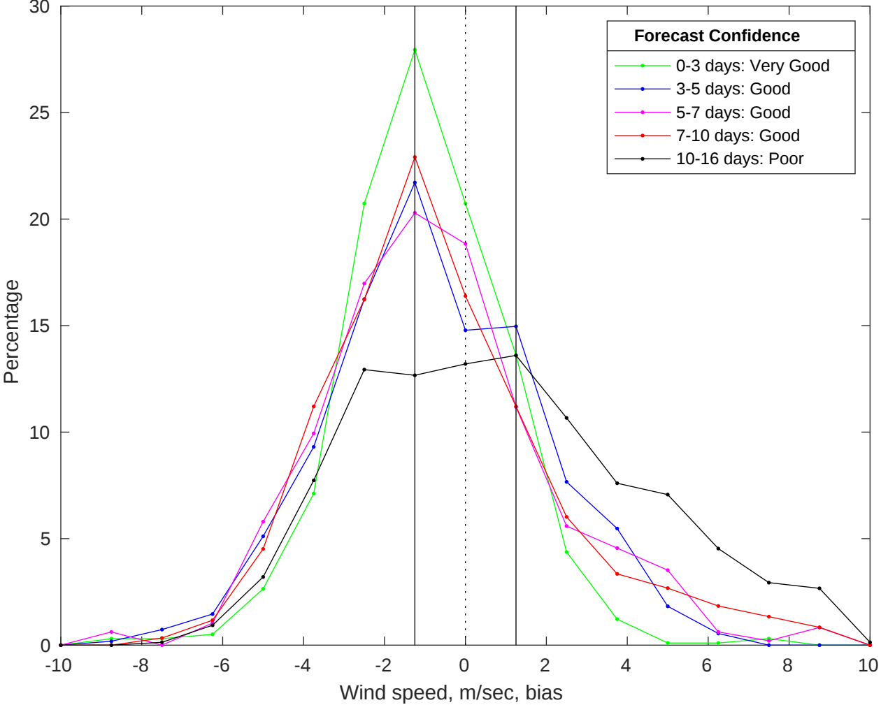
NDBC 46028 vs GFS Winds Bias Histogram: 23-Jan-2026
