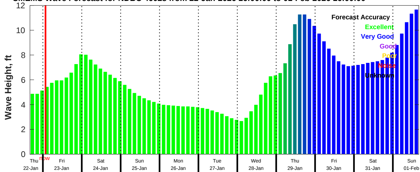
CMEMS Wave Forecast for NDBC 46028 from 22-Jan-2026 16:00:00 to 01-Feb-2026 16:00:00
