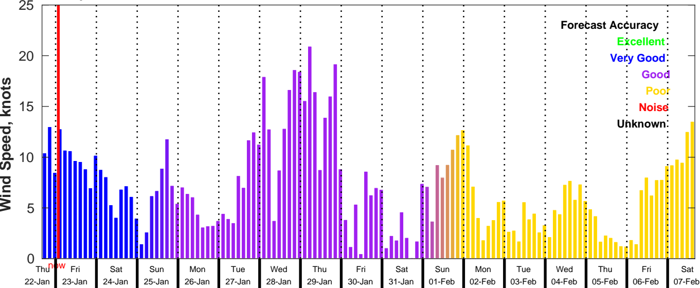
GFS Wind Speed Forecast for NDBC 46028 from 22-Jan-2026 16:00:00 to 07-Feb-2026 16:00:00
