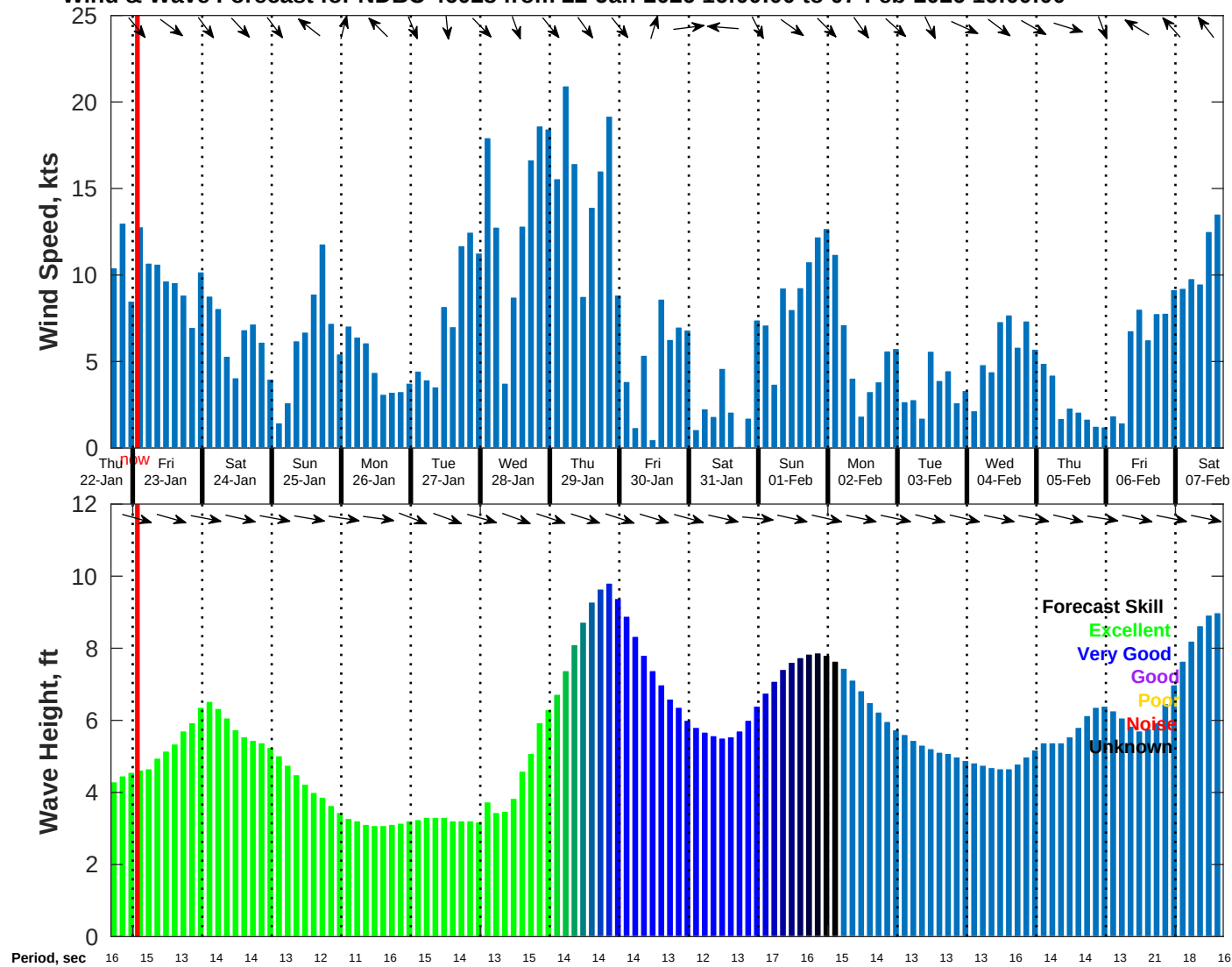
Wind & Wave Forecast for NDBC 46028 from 22-Jan-2026 16:00:00 to 07-Feb-2026 16:00:00
