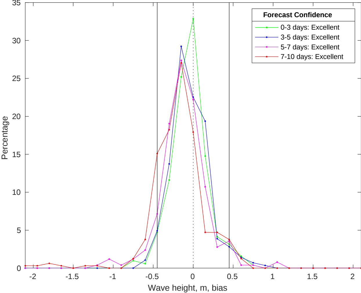
NDBC 46054 vs CMEMS Waves Bias Histogram: 23-Jan-2026
