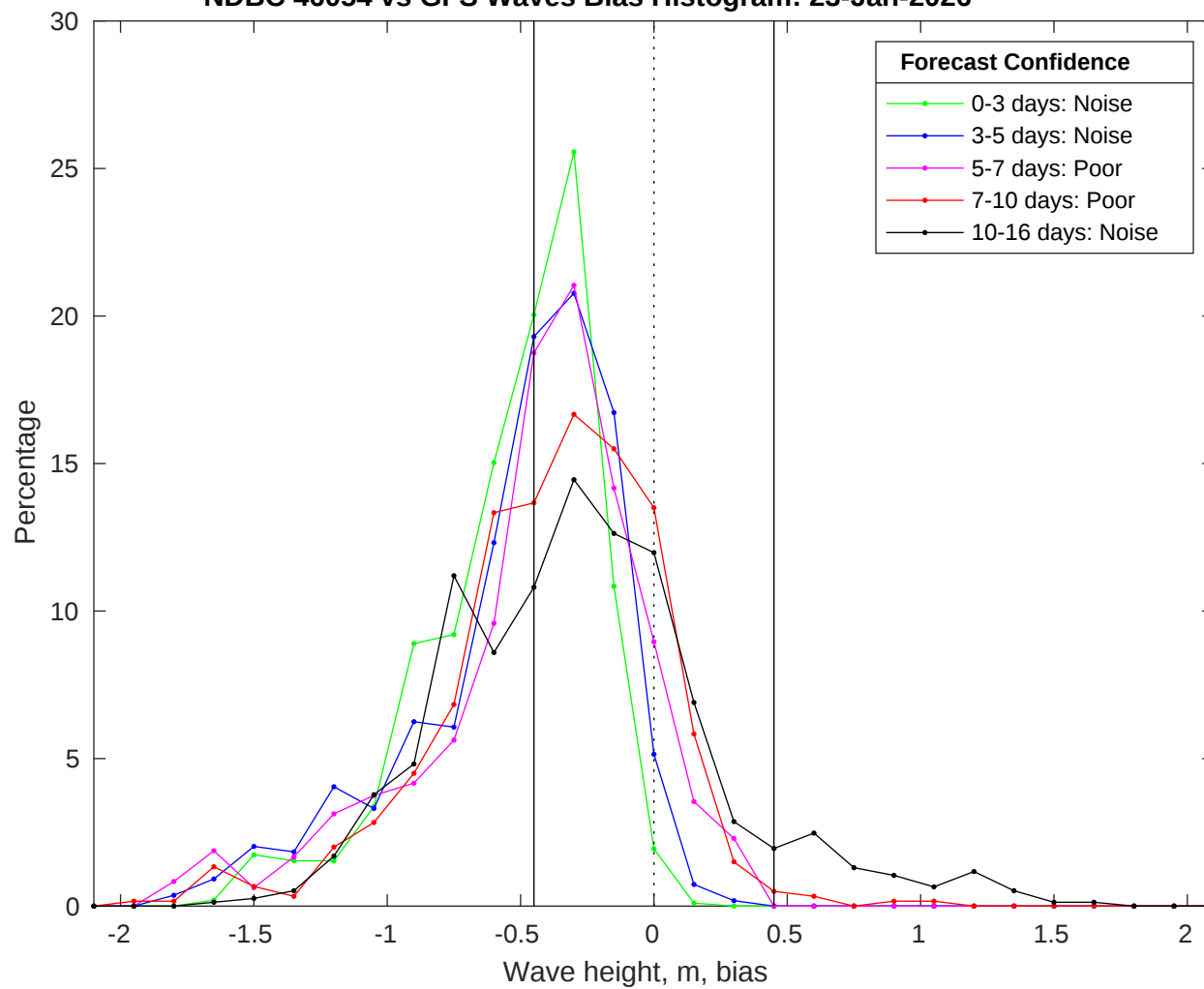
NDBC 46054 vs GFS Waves Bias Histogram: 23-Jan-2026
