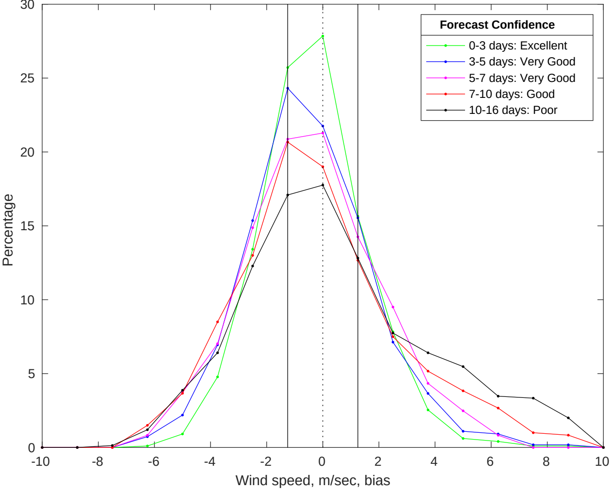
NDBC 46054 vs GFS Winds Bias Histogram: 23-Jan-2026
