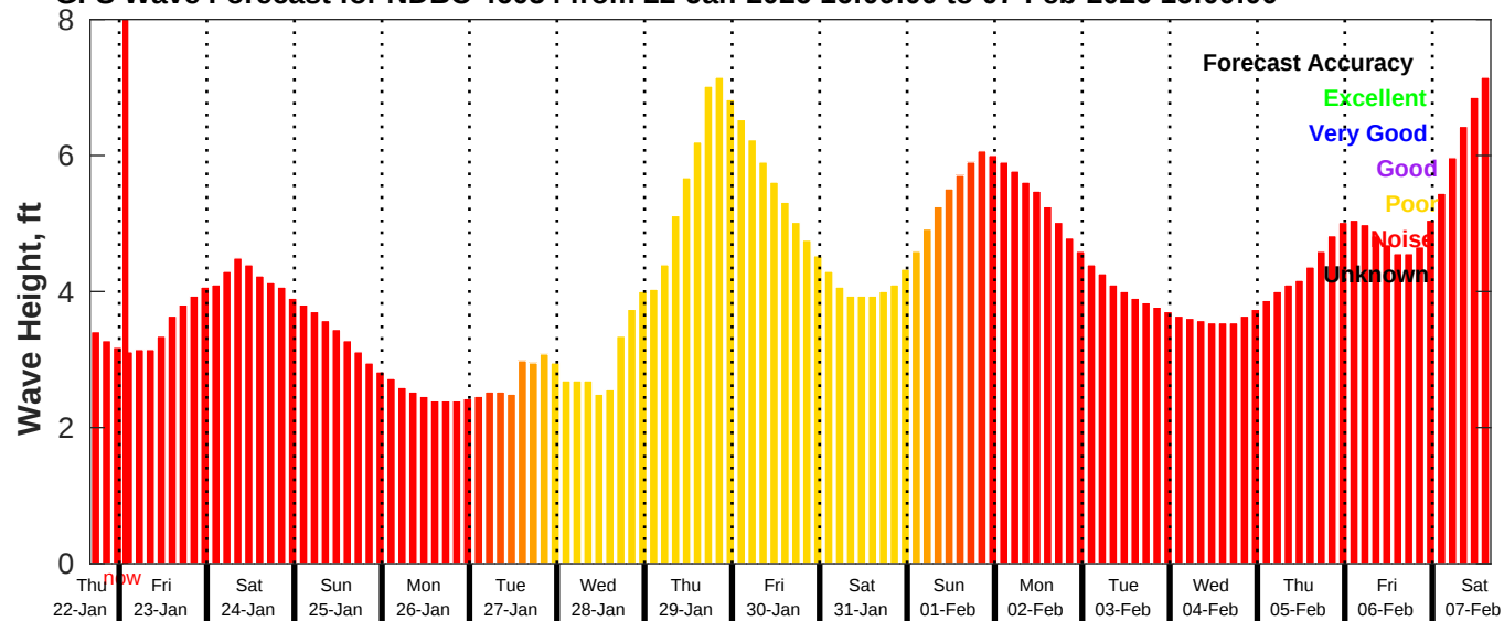
GFS Wave Forecast for NDBC 46054 from 22-Jan-2026 16:00:00 to 07-Feb-2026 16:00:00
