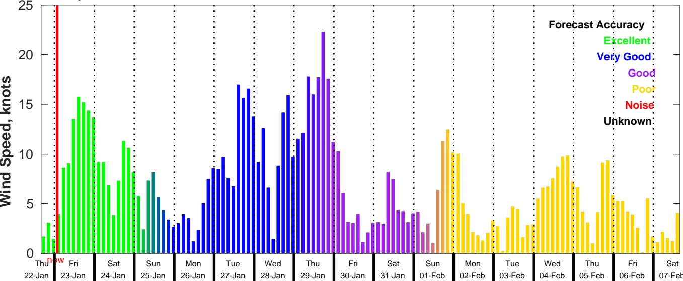
GFS Wind Speed Forecast for NDBC 46054 from 22-Jan-2026 16:00:00 to 07-Feb-2026 16:00:00
