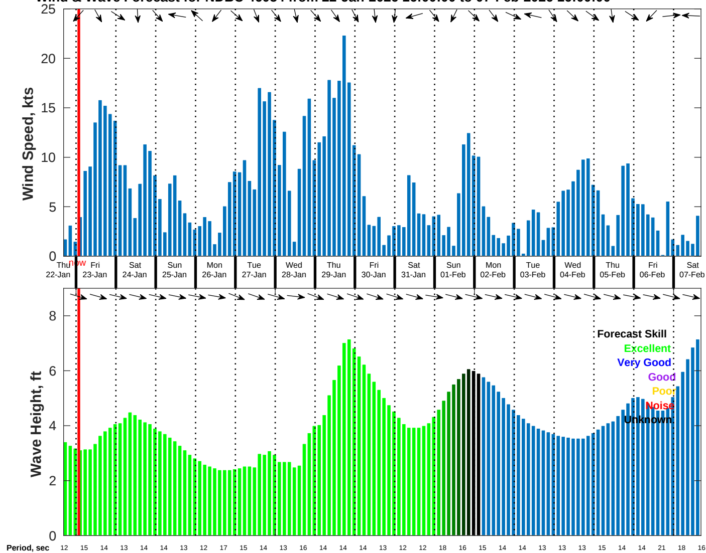
Wind & Wave Forecast for NDBC 46054 from 22-Jan-2026 16:00:00 to 07-Feb-2026 16:00:00
