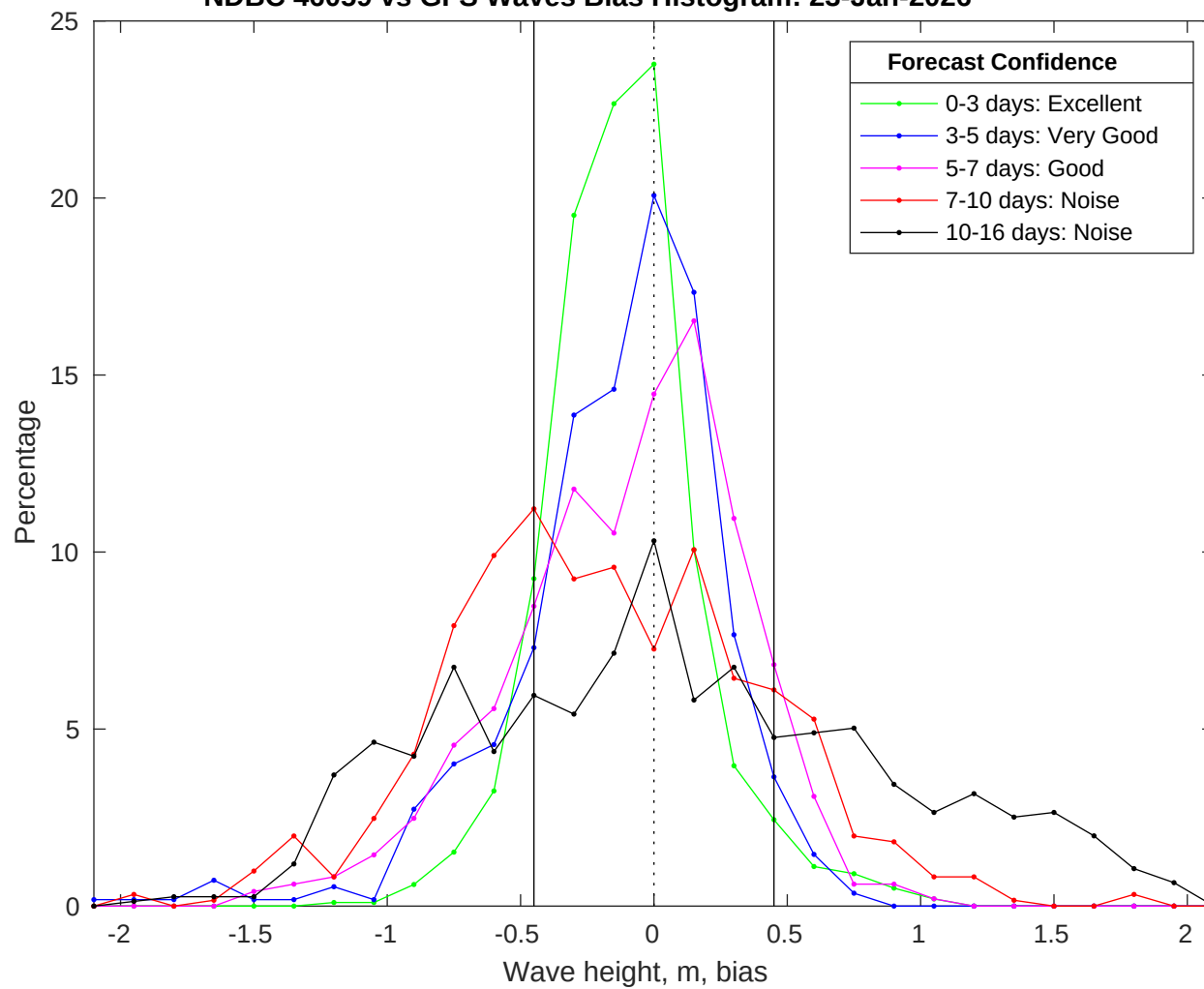
NDBC 46059 vs GFS Waves Bias Histogram: 23-Jan-2026
