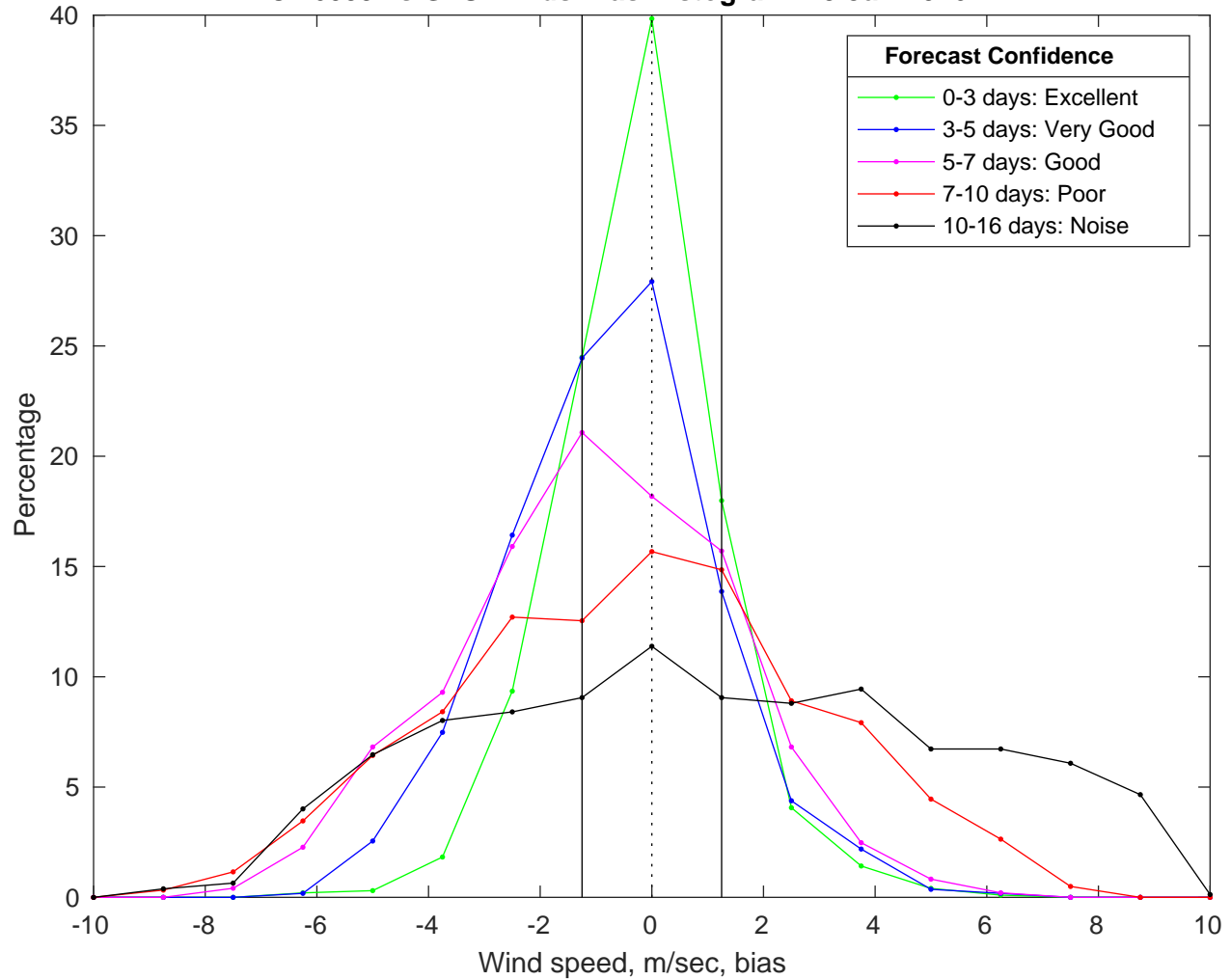
NDBC 46059 vs GFS Winds Bias Histogram: 23-Jan-2026
