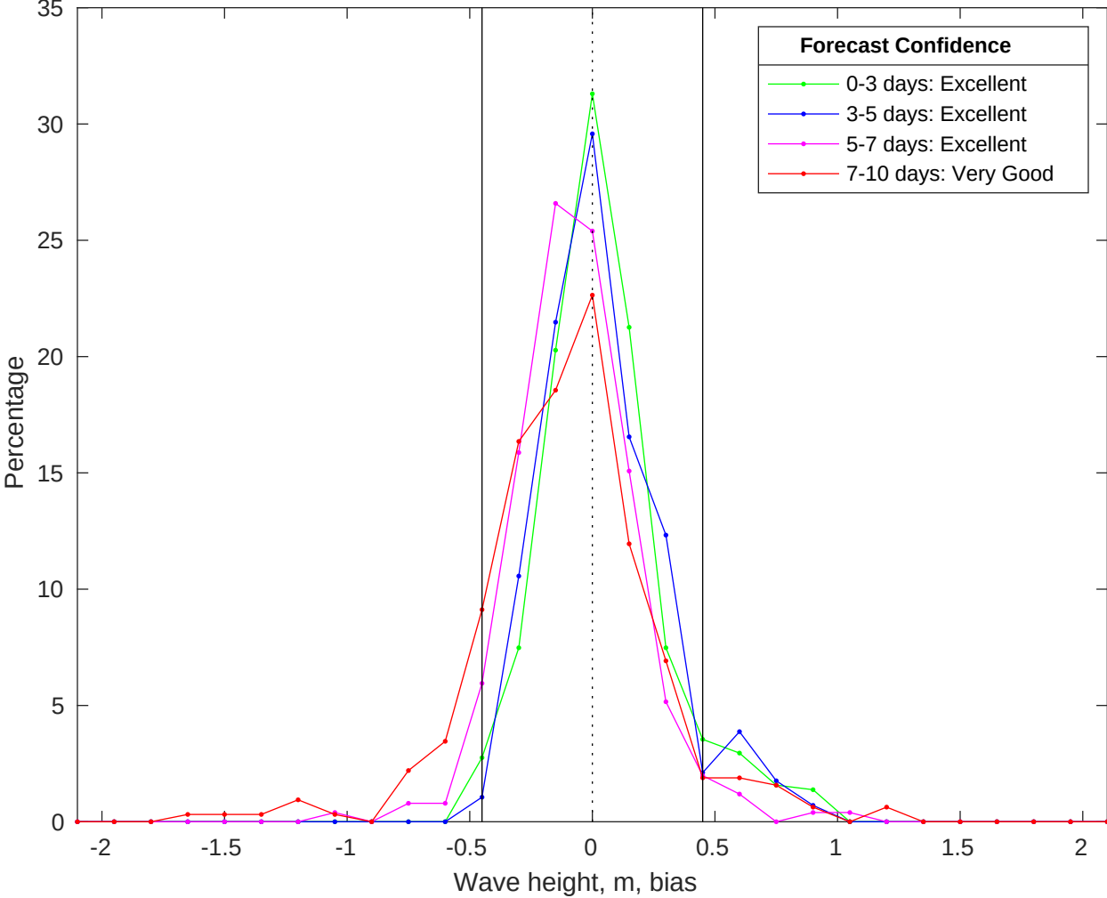
NDBC 46069 vs CMEMS Waves Bias Histogram: 23-Jan-2026
