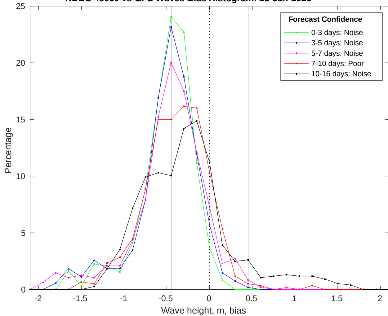
NDBC 46069 vs GFS Waves Bias Histogram: 23-Jan-2026
