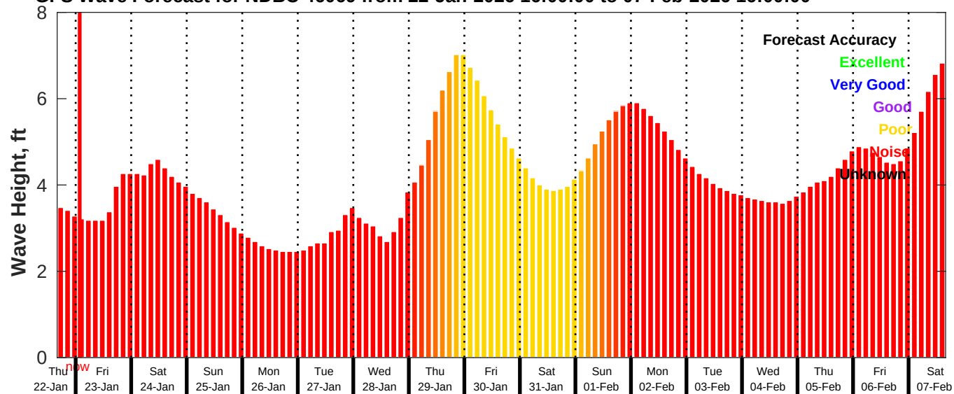
GFS Wave Forecast for NDBC 46069 from 22-Jan-2026 16:00:00 to 07-Feb-2026 16:00:00
