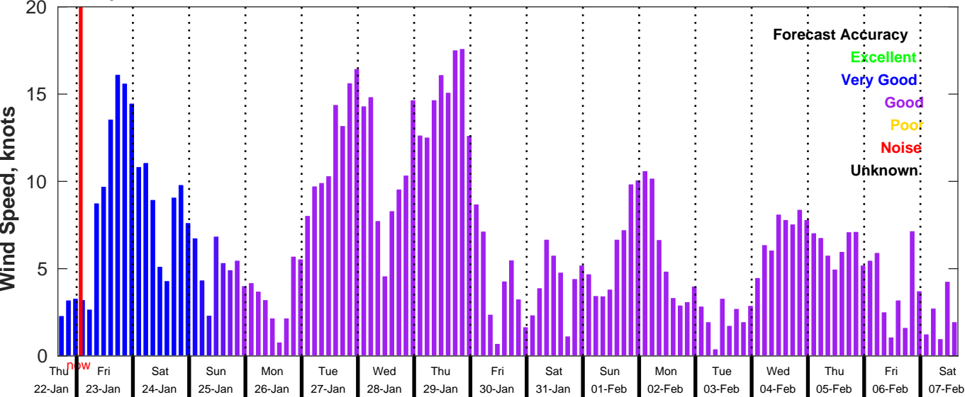
GFS Wind Speed Forecast for NDBC 46069 from 22-Jan-2026 16:00:00 to 07-Feb-2026 16:00:00
