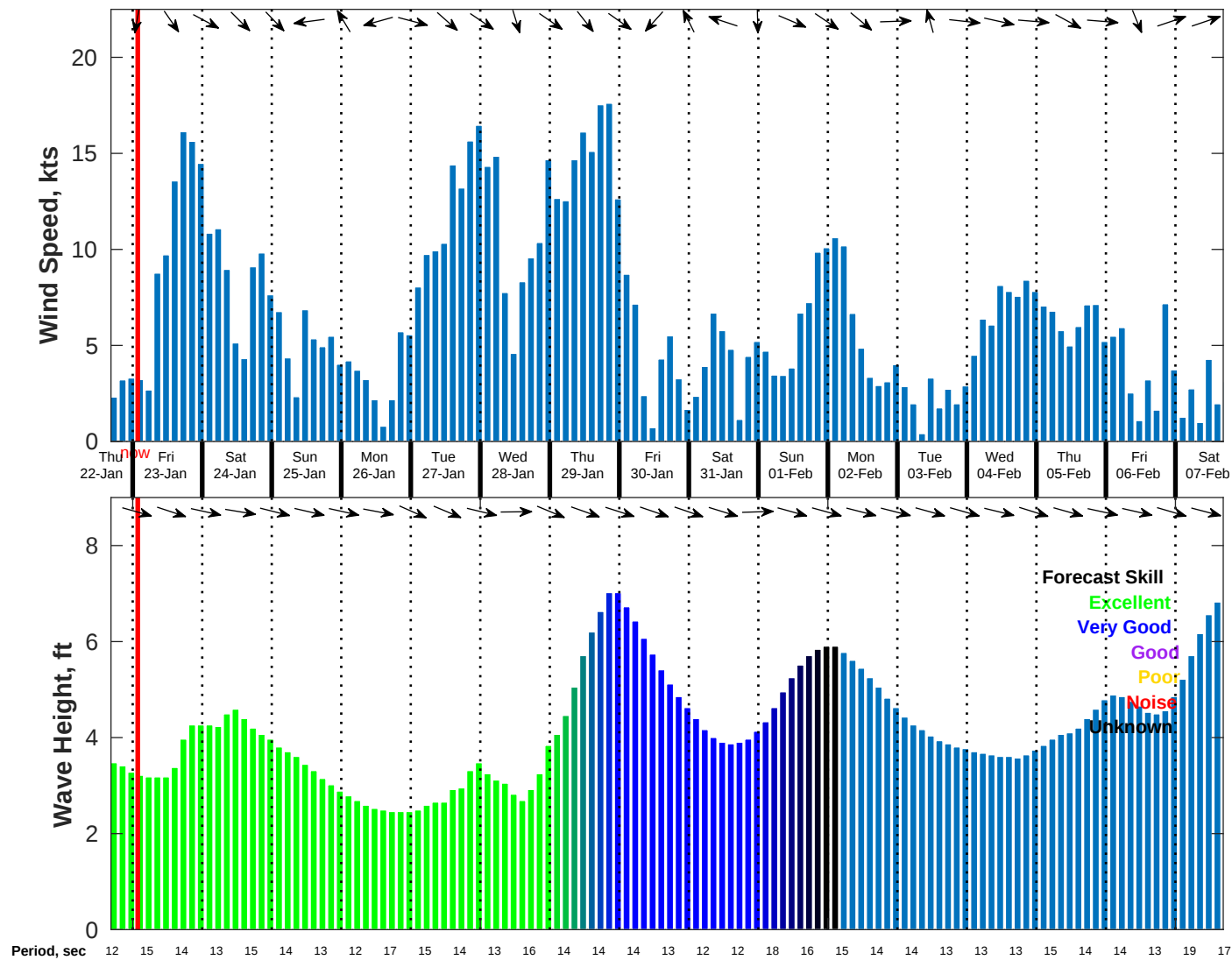
Wind & Wave Forecast for NDBC 46069 from 22-Jan-2026 16:00:00 to 07-Feb-2026 16:00:00
