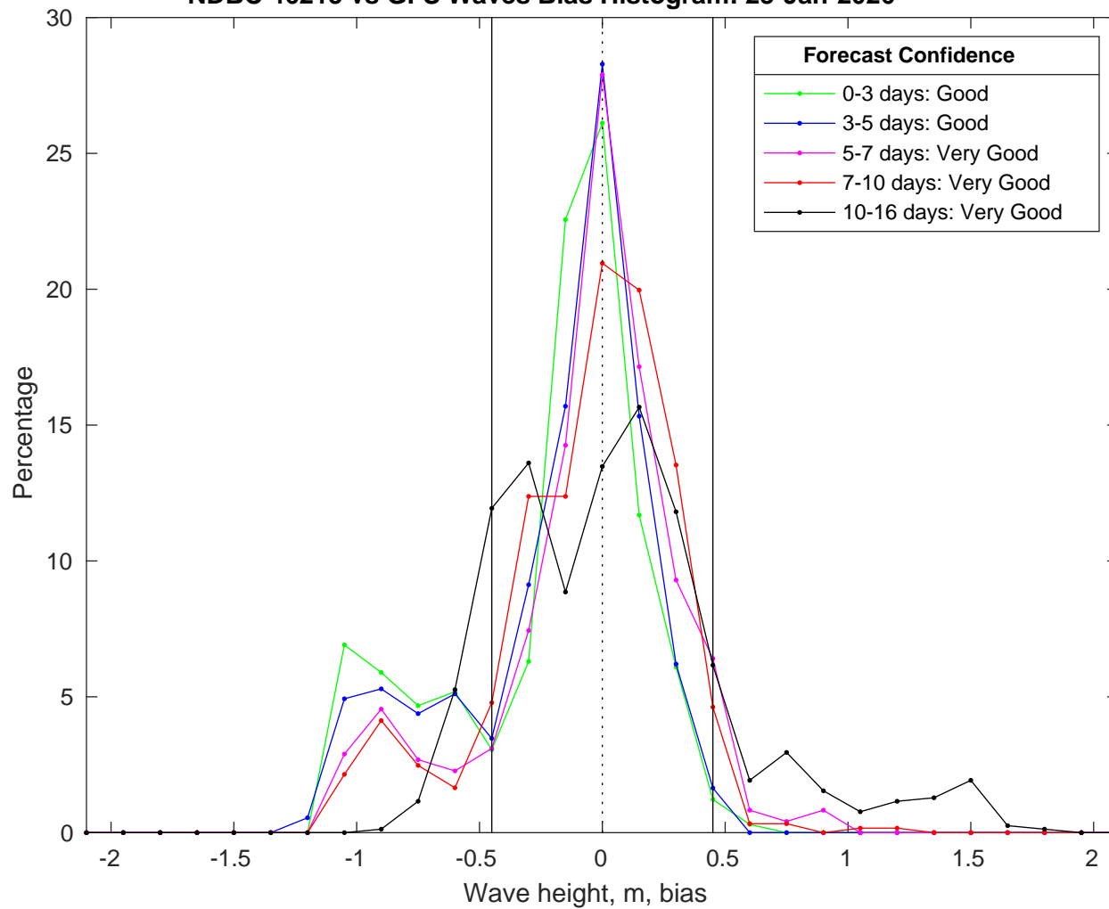
NDBC 46215 vs GFS Waves Bias Histogram: 23-Jan-2026
