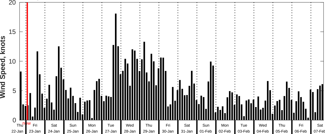
GFS Wind Speed Forecast for NDBC 46215 from 22-Jan-2026 16:00:00 to 07-Feb-2026 16:00:00
