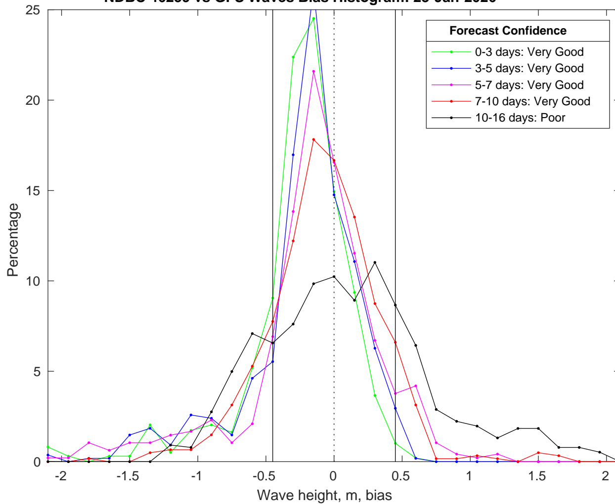
NDBC 46259 vs GFS Waves Bias Histogram: 23-Jan-2026
