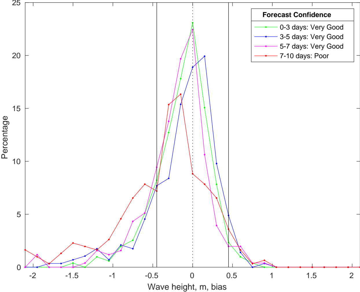
NDBC 51000 vs CMEMS Waves Bias Histogram: 23-Jan-2026
